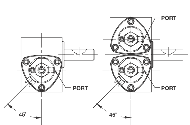
"ACT" & "CT" FOR 3/4 BORE
