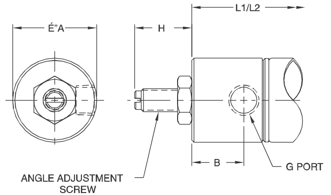
Angle Adjustment (A Option)
