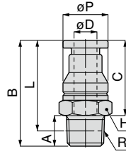
Taper thread
