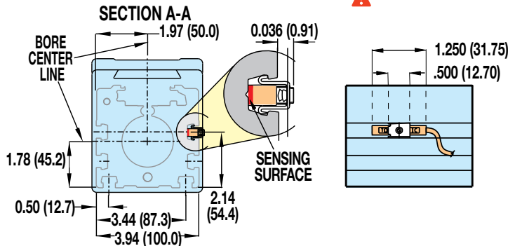
OPTIONAL SWITCH MOUNTING
