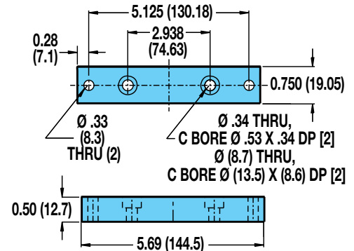
OPTIONAL MOUNTING PLATES
