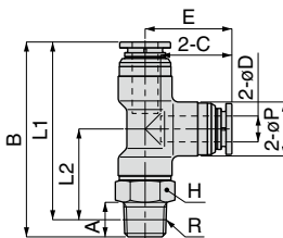
Taper pipe thread
