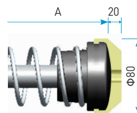
Urethane Cap
