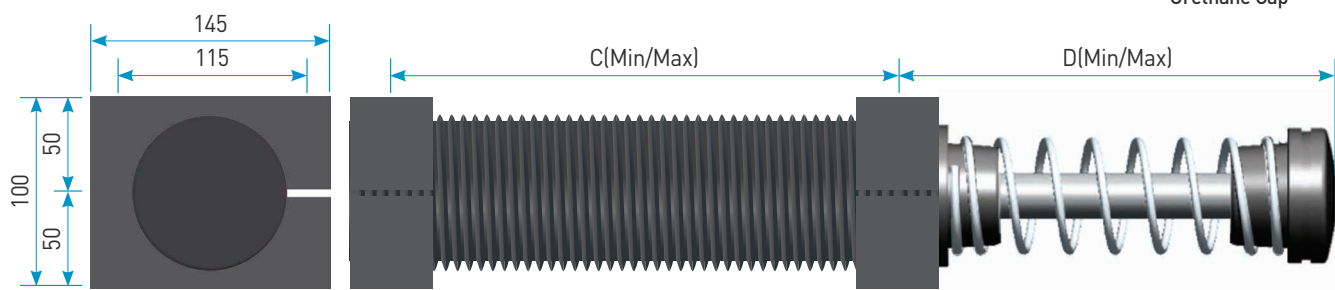
Urethane Cap
